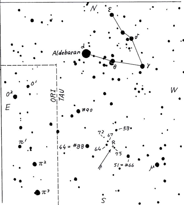
AAVSO (b) chart
