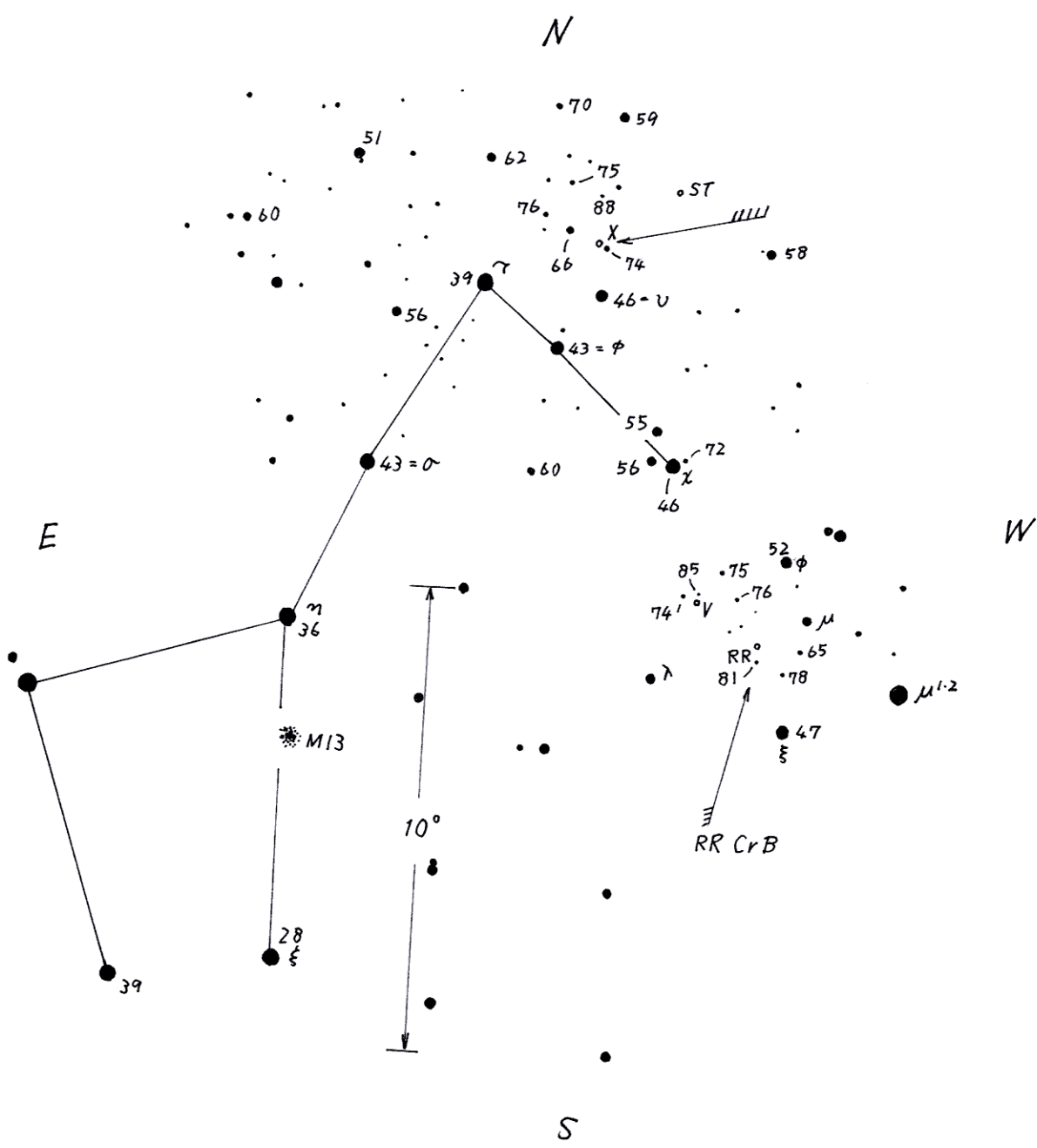
AAVSO (a) Chart
