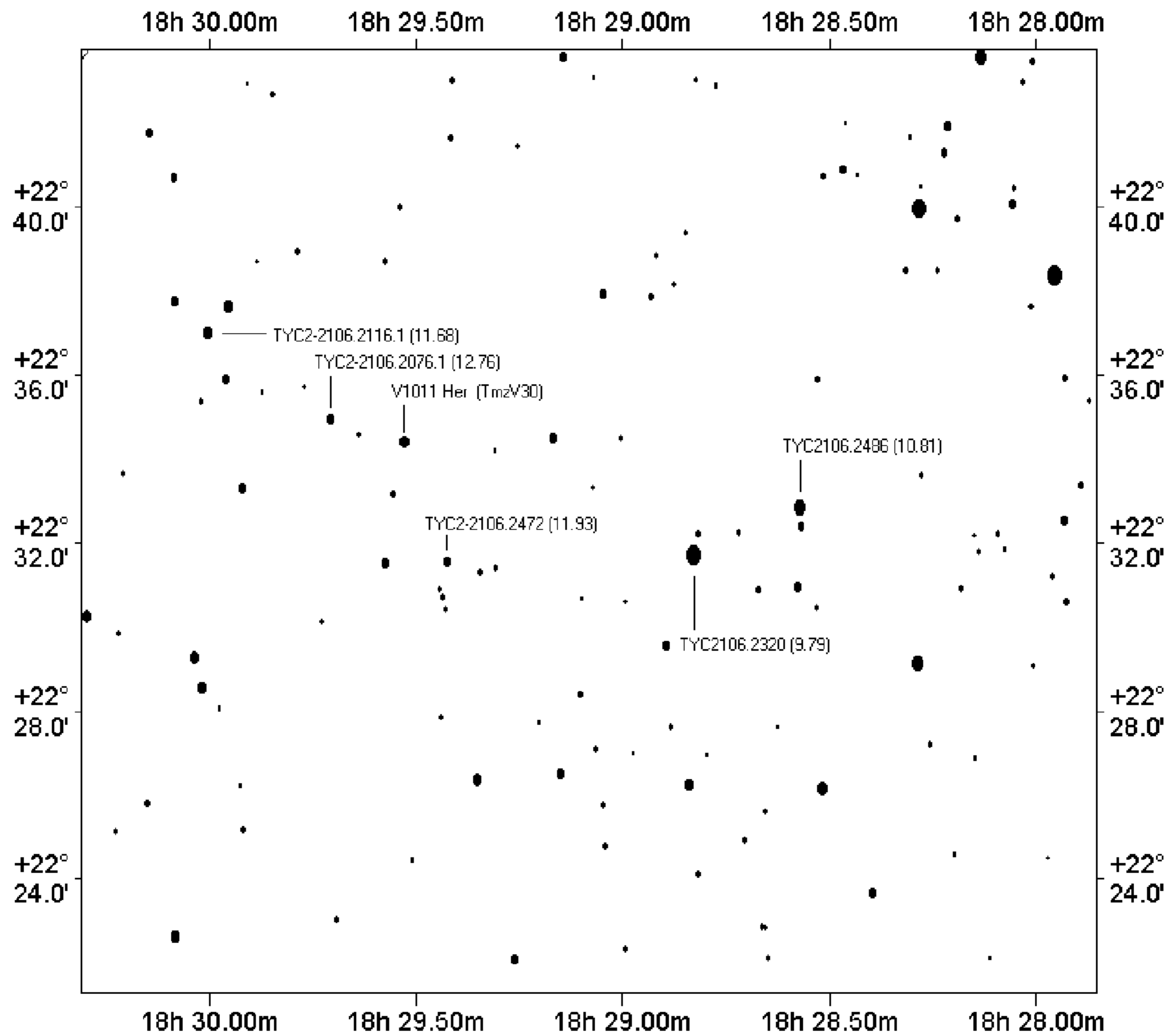
V1011 Her (TmzV30) EA 10.4-11.6(P) 18h29m31.4s +22d34'25"(2000)
